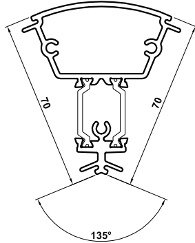
ETC385 135° Corner Post
